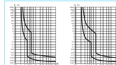
Diagram 1 Type B Thermal/Electromagnetic tripping curve
