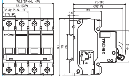
Figure 4. Overall and Installation dimensions of MC
