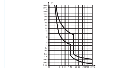
Diagram 3 Type D Thermal/Electromagnetic tripping curve
